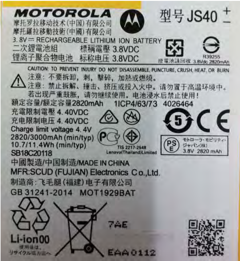
电池组铭牌 Battery Nameplate
